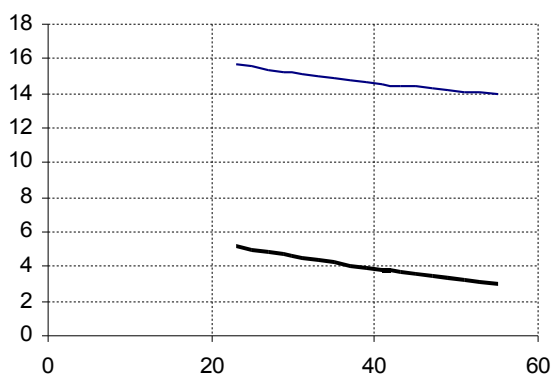
Figure 3. Dependence of oil watering from the demulsifying agent consumption (upper curve – at t_d = 35 °C, lower – at t_d = 50 °C)
