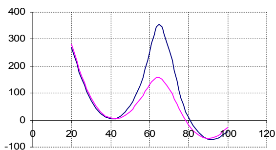
Figure 7. Dependence of technological profit from temperature in device (upper curve – at demulsifying agent consumption 35 g/t, lower - at 23 g/t)
