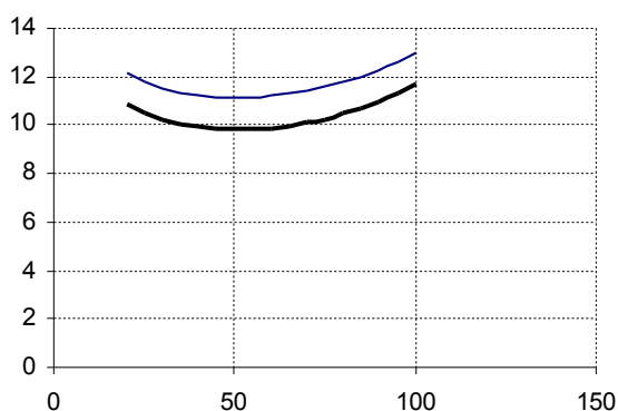
Figure 5. Dependences of total expenses from temperature in device (upper curve – at demulsifying agent consumption 35 g/t, lower - at 23 g/t)
