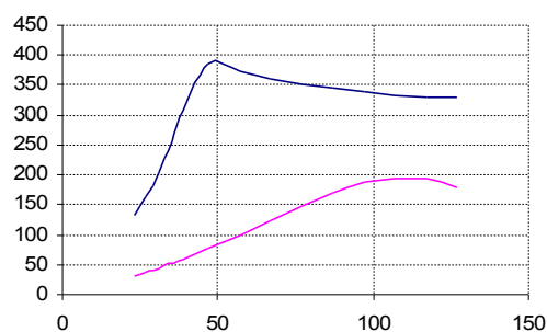
Figure 8. Dependence of technological profit from demulsifying agent consumption (upper curve – at t_d = 60 °C, lower – at t_d = 50 °C)
