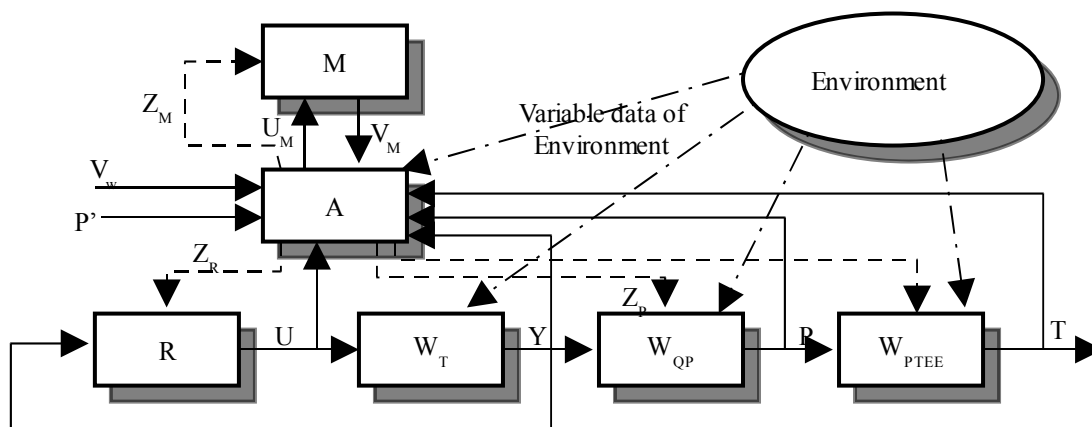
Figure 1. Structure of the adaptive control system
