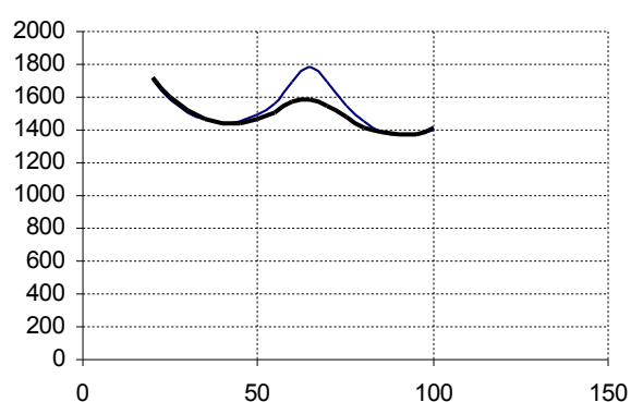
Figure 6. Dependence of technological receipts from temperature in device (upper curve – at demulsifying agent consumption 35 g/t, lower - at 23 g/t)
