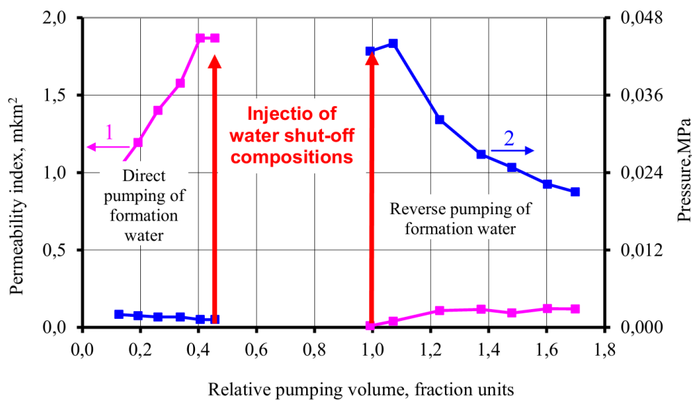
Fig. 3. Behavior of pumping pressure and permeability of water-saturated reservoir model after its treatment with 50 % water solution “OVP-1”: 1 – permeability factor; 2 – pumping pressure
