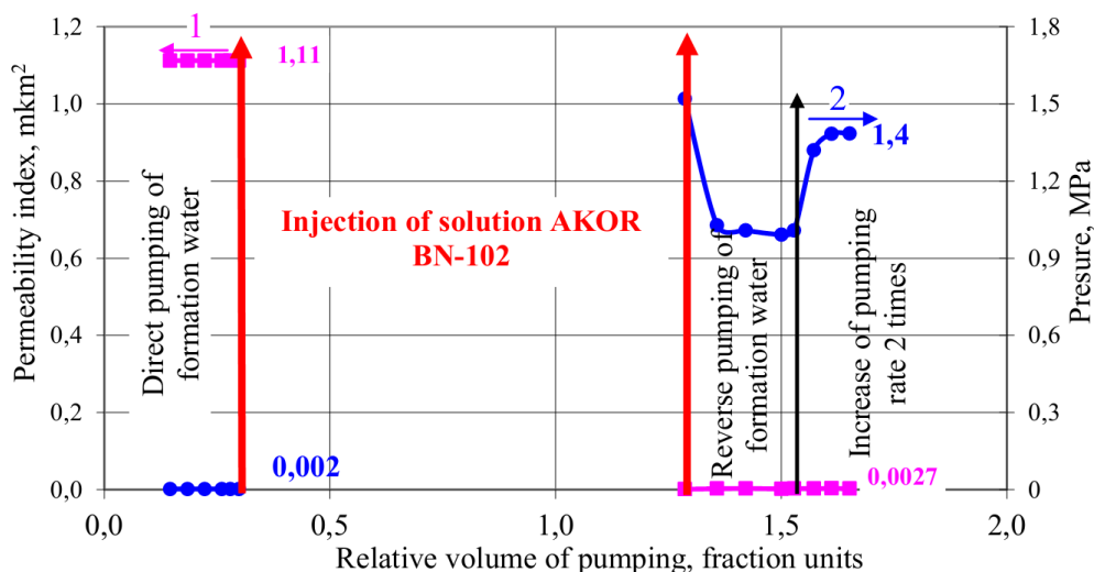
Fig. 1. Behavior of pumping pressure and permeability of water-saturated reservoir model after its treatment with water shut-off compositions based on “AKOR-BN102”:
