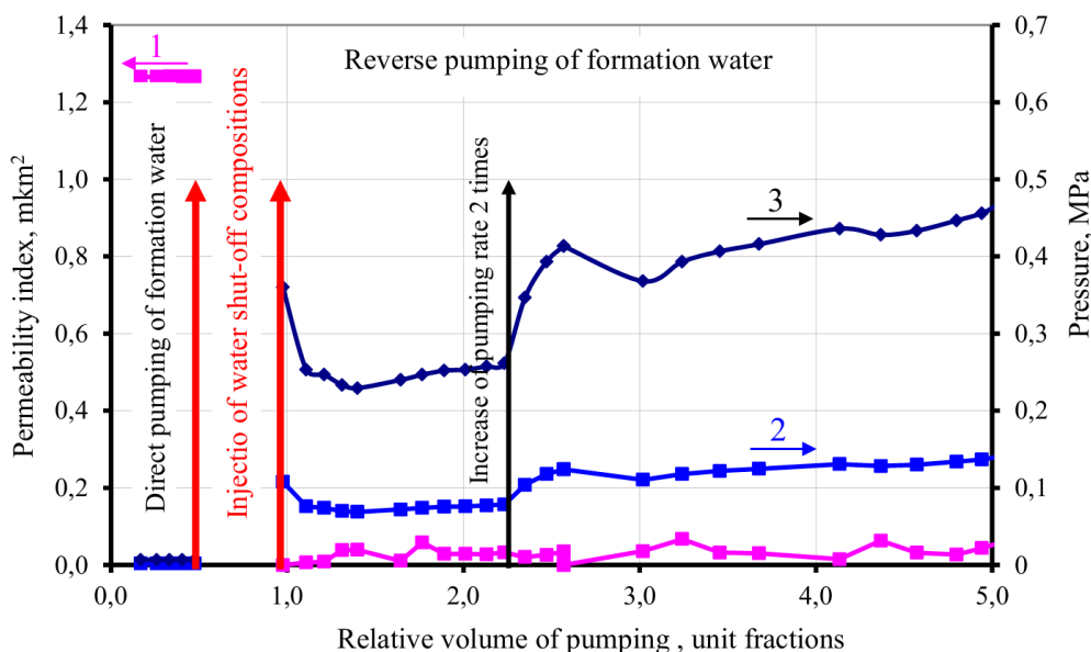
Fig. 2. Behavior of permeability, pressure gradient and pumping pressure after pumping into a water-saturated reservoir model water shut-off compositions based on “GPAN” and mineralized water ( \rho = 1,15 \text{ g/cm}^3 ):
