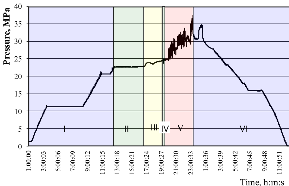
Fig. 4. Behavior of bottomhole pressure while injecting water shut-off compositions into well 45 of Dubrovskoye oil field without pulsing (section III) and in pulsing (section V) mode: sections I and VI – respectively running in and running out of the assembly; II and IV – preliminary works
