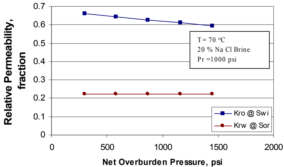
Figure 11. The effect of net overburden pressure on oil and water relative permeability at the end points
